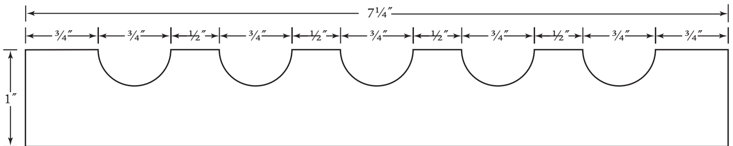
FL714B Five \frac{3}{4} " flutes, \frac{1}{2} " spacing, 7\frac{1}{4} " wide
