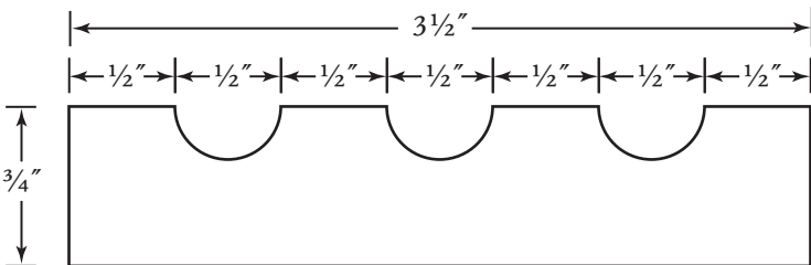
FL312B 1/2" flutes, 1/2" spacing, 3 1/2" wide
