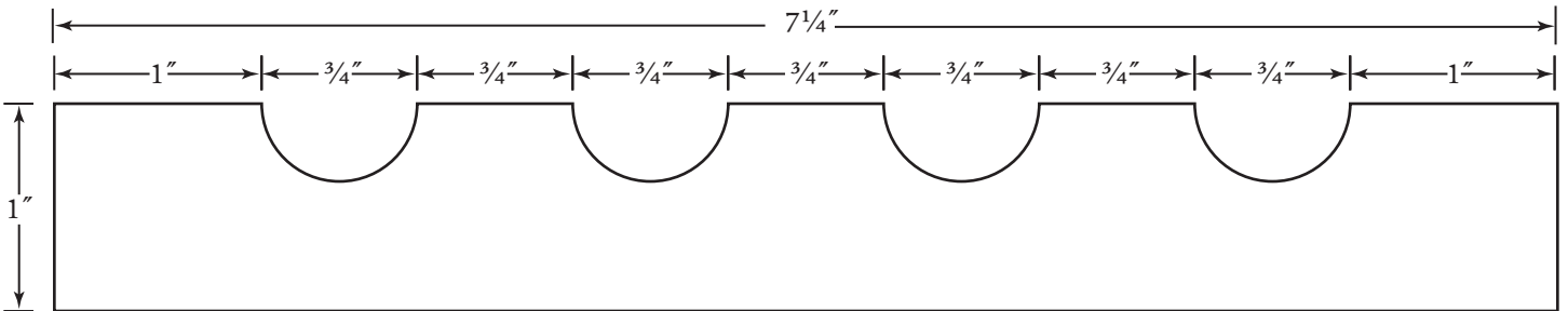
FL714C Four \frac{3}{4} " flutes, \frac{3}{4} " spacing, 7\frac{1}{4} " wide
