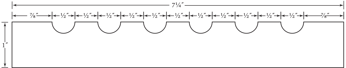
FL714A Six \frac{1}{2} " flutes, \frac{1}{2} " spacing, 7\frac{1}{4} " wide
