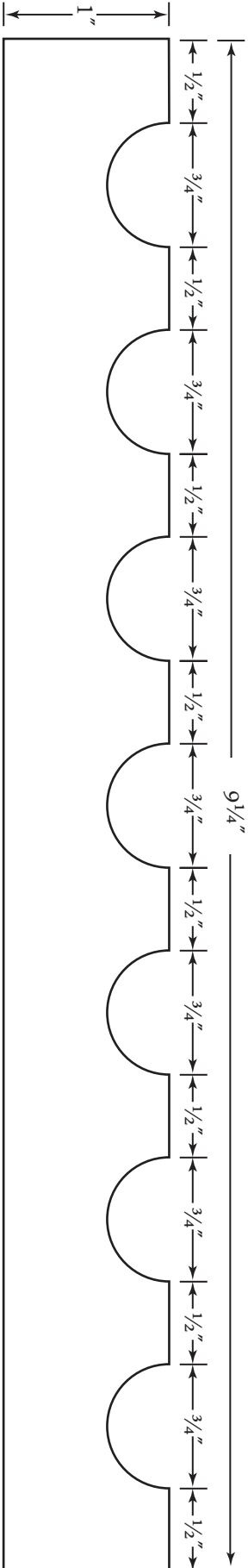
FL914B Seven 3/4 " flutes, 1/2 " spacing, 9\frac{1}{4} " wide
