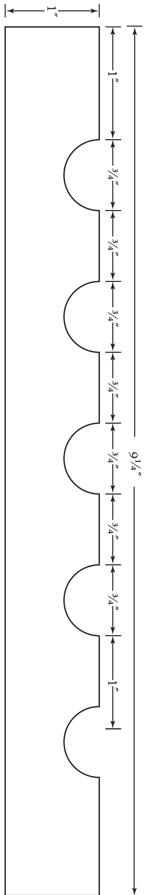
FL914A Six 3/4 " flutes, 3/4 " spacing, 9\frac{1}{4} " wide
