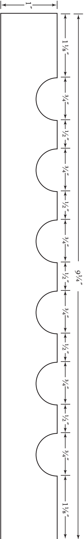
FL914C Six 3/4 " flutes, 1/2 " spacing, 9\frac{1}{4} " wide
